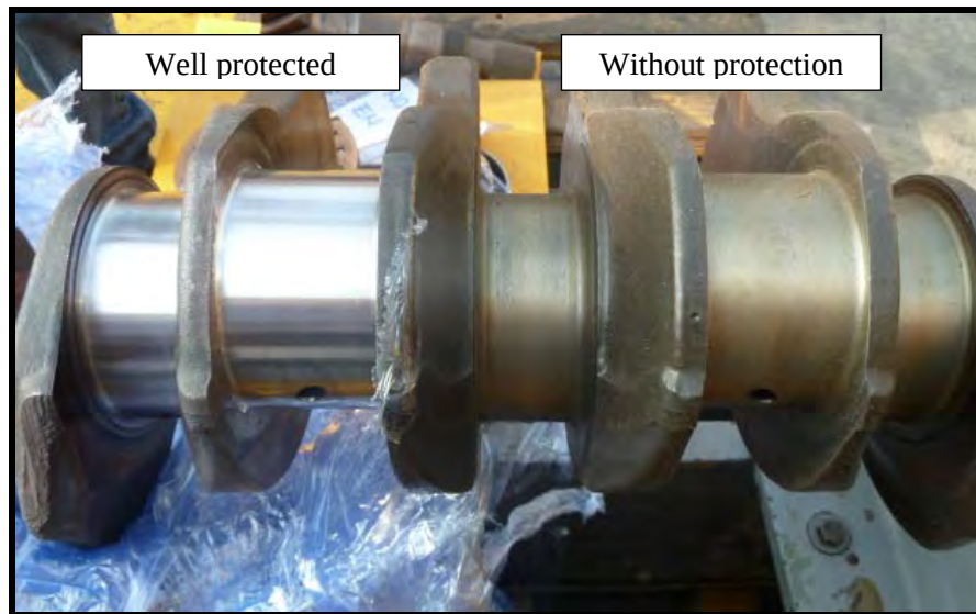
Figure 3. Crankshaft after removed of the VCI Stretch Film
