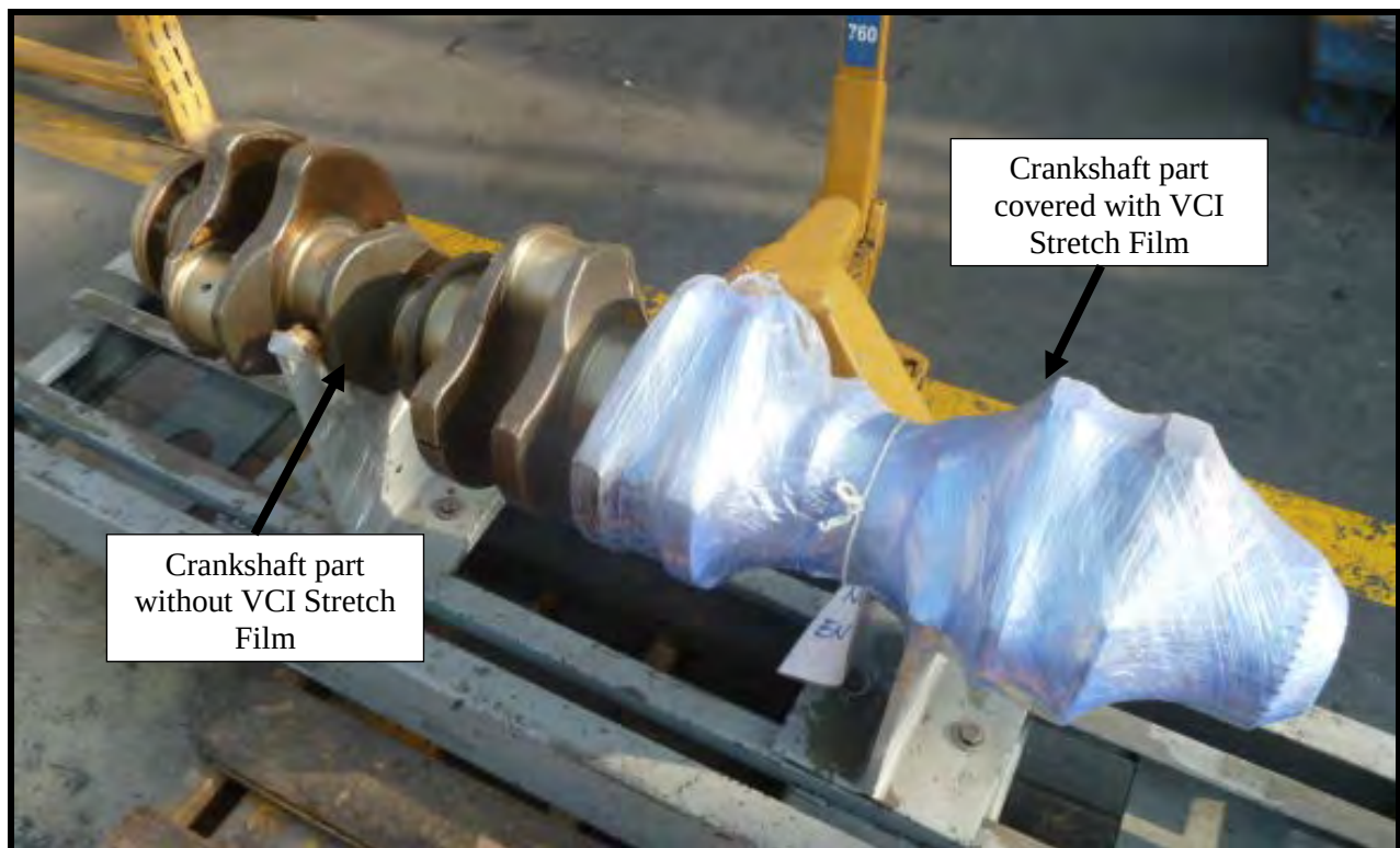
Figure 2. Example of crankshaft protected with VCI Stretch Film
